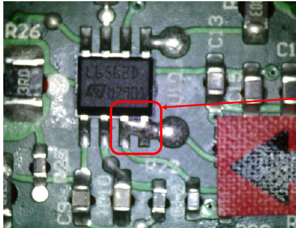
Solder Bridge, bottom side U10
