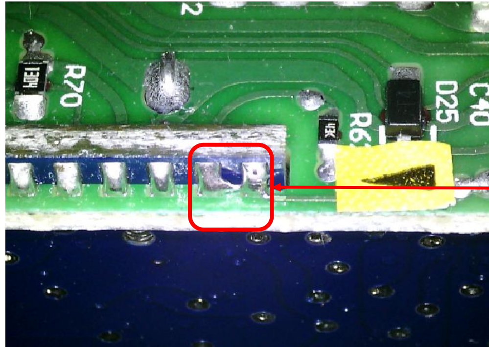
Solder Bridge, bottom side DC1
