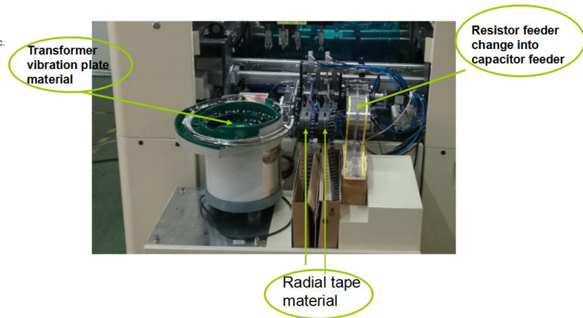
Odd Form Insertion Machine Appearance
