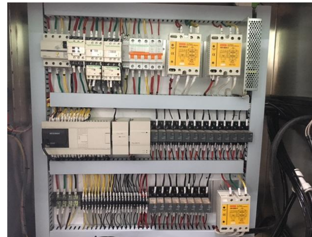
Control Unit
